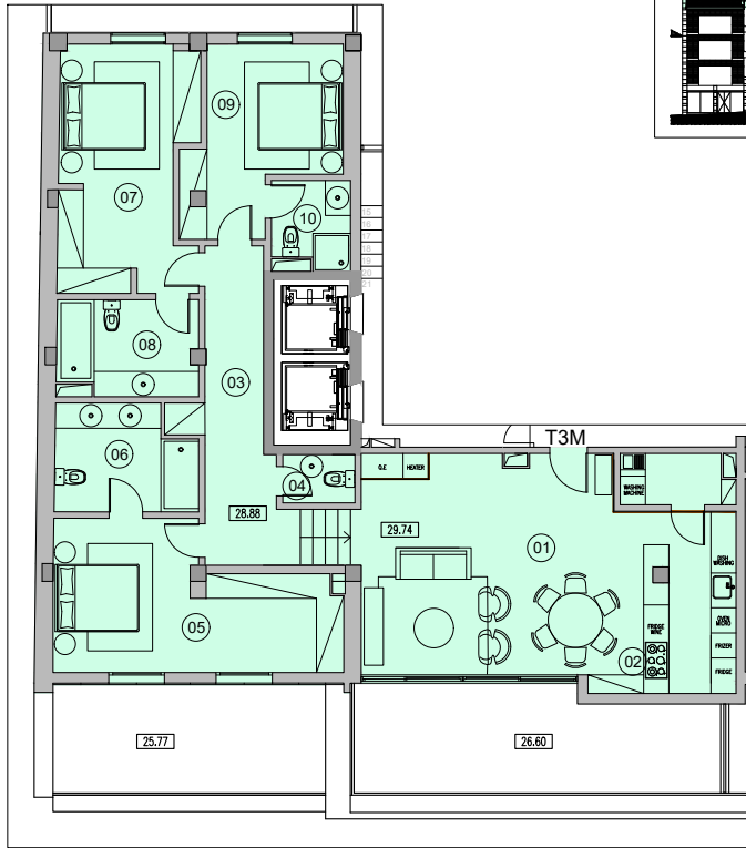
Apartment floor plan
