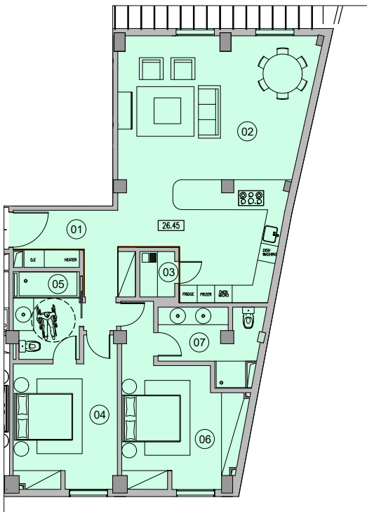
Apartment floor plan
